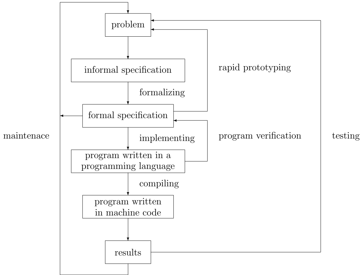
Figure 1: A software life-cycle model illustrating abstraction
